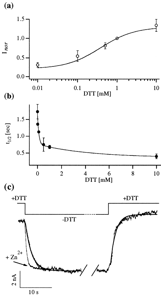
Fig. 2. Reversible current increase and kinetic of activation in P. oceanica vacuoles as a function of DTT concentration. a: Normalised current, I_{nor} = I(\text{DTT})/I(\text{DTT} = 1 \text{ mM}) , plotted together with the best fit obtained by the Michaelis-Menten function I_{nor} = k_0 + k_1[\text{DTT}]/([\text{DTT}] + K_m) (continuous line), where k_0 = 0.20 \pm 0.04 , k_1 = 1.09 \pm 0.14 and K_m = 0.38 \pm 0.18 mM. b: Time constant of half activation, t_{1/2} , as a function of DTT concentration. Step potentials to +40 mV or to +80 were applied from a holding potential of 0 mV. The amplitude of the step potential did not affect t_{1/2} appreciably. The continuous line through the experimental data points has no theoretical meaning. c: Typical reversible decrease/increase of P. oceanica current observed on the removal/addition of DTT by the fast perfusion procedure. The increase and decrease of the steady-state current followed an exponential course with time constants of \sim 2 s. Steady-state voltage at +80 mV. The arrow indicates the decrease of the current (appropriately scaled) induced by the addition of 1 mM \text{ZnCl}_2 ; applied voltage +100 mV. Note that the inhibition of the current induced by \text{Zn}^{2+} is reported uniquely to show the velocity of the fast perfusion system. The upper profile represents the presence/absence of 1 mM DTT.
